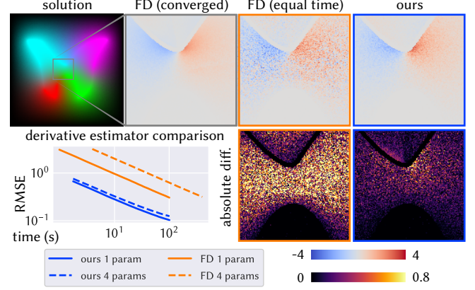
Figure 6. Finite-difference (FD) approximations of derivatives (middle-right) require only primary walks, but scale poorly with parameter count. Differential WoS (far-right) instead computes derivatives for all parameters \pi with a single differential walk, leading to less noisy results at equal time.
