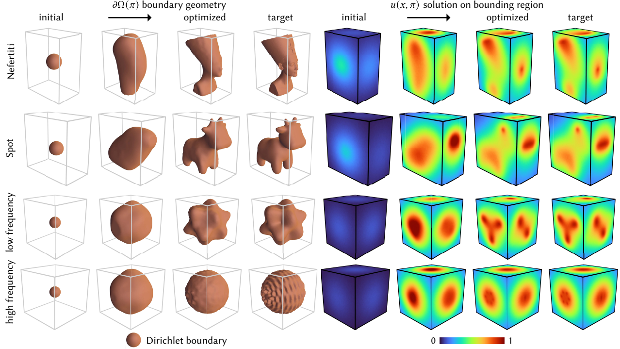
Figure 10. Inspired by shape-from-diffusion applications, we use measurements on a bounding box ( far right, column ) to evolve 3D models starting from a sphere ( left ). As with any reconstruction through a diffusive medium, high-frequency surface details have negligible influence on the solution, and are therefore not captured in the reconstructions ( bottom row ).
