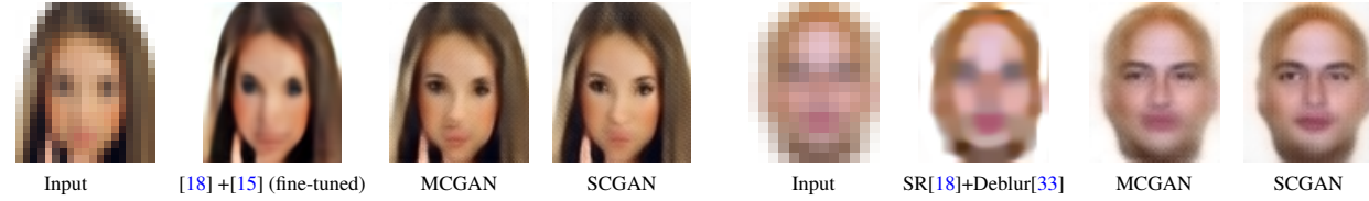
Figure 7. Results on real face images. Our method generates more realistic-looking faces, especially around the eye and mouth regions.
