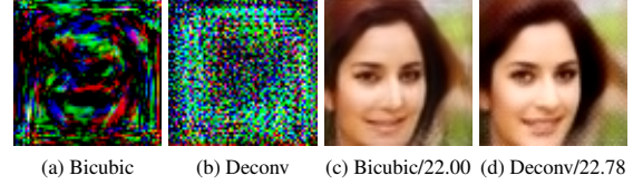
Figure 10. Analyzing the checkerboard artifacts. (a) and (b) are the output of randomly initialized generators with bicubic and deconvolution layers respectively. Using bicubic interpolation for upsampling (c) reduces the artifacts but has lower PSNR than deconvolutional (d). See Figure 1 for the input and ground truth.
