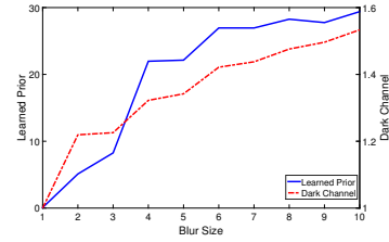
Figure 8. The learned discriminator favors clear images over blurred ones, similar to the empirical dark channel prior. We blur clear images from CelebA [26] using horizontal motion blur kernels ranging from 2 to 10 pixels and evaluate the learned discriminator -\sum \log D(I_i) . The left y-axis represents the energy of the learned prior. The right y-axis shows the energy of the dark channel prior on blurry images relative to that on clear images.
